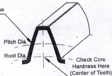
Gear Profile
